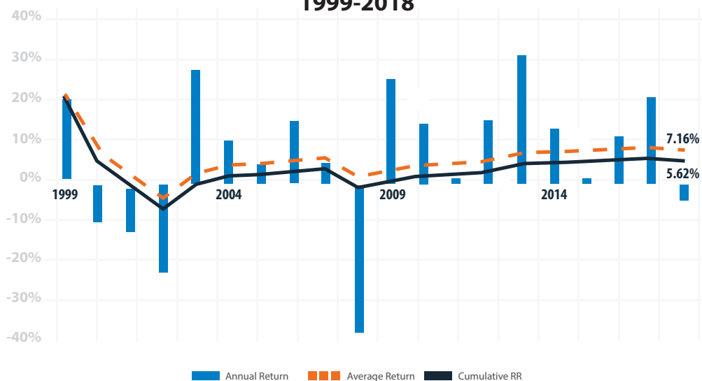
S&P 500 Return (Including Dividends) 1999-2018
